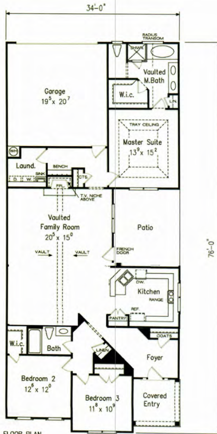
FLOOR PLAN
